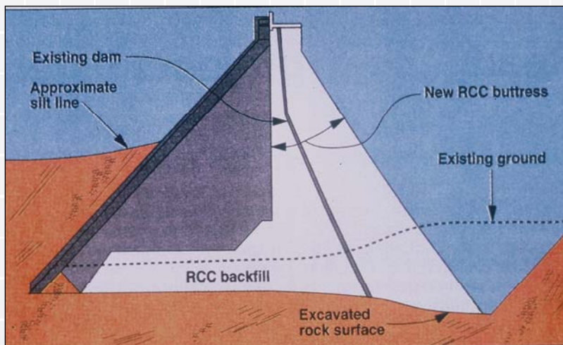
Littlerock Dam – California
