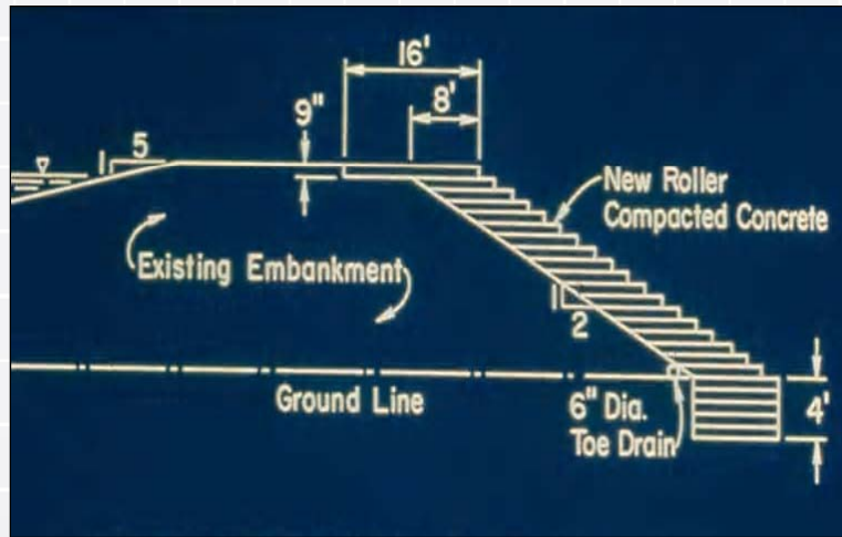
Brownwood County Club Dam – Texas
