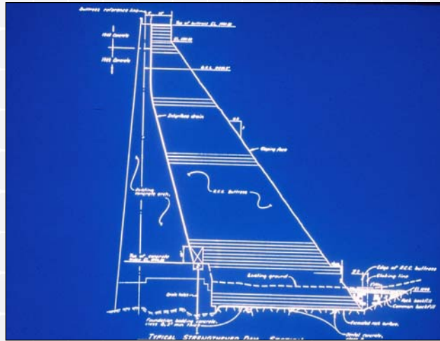
Gibraltar Dam – California
